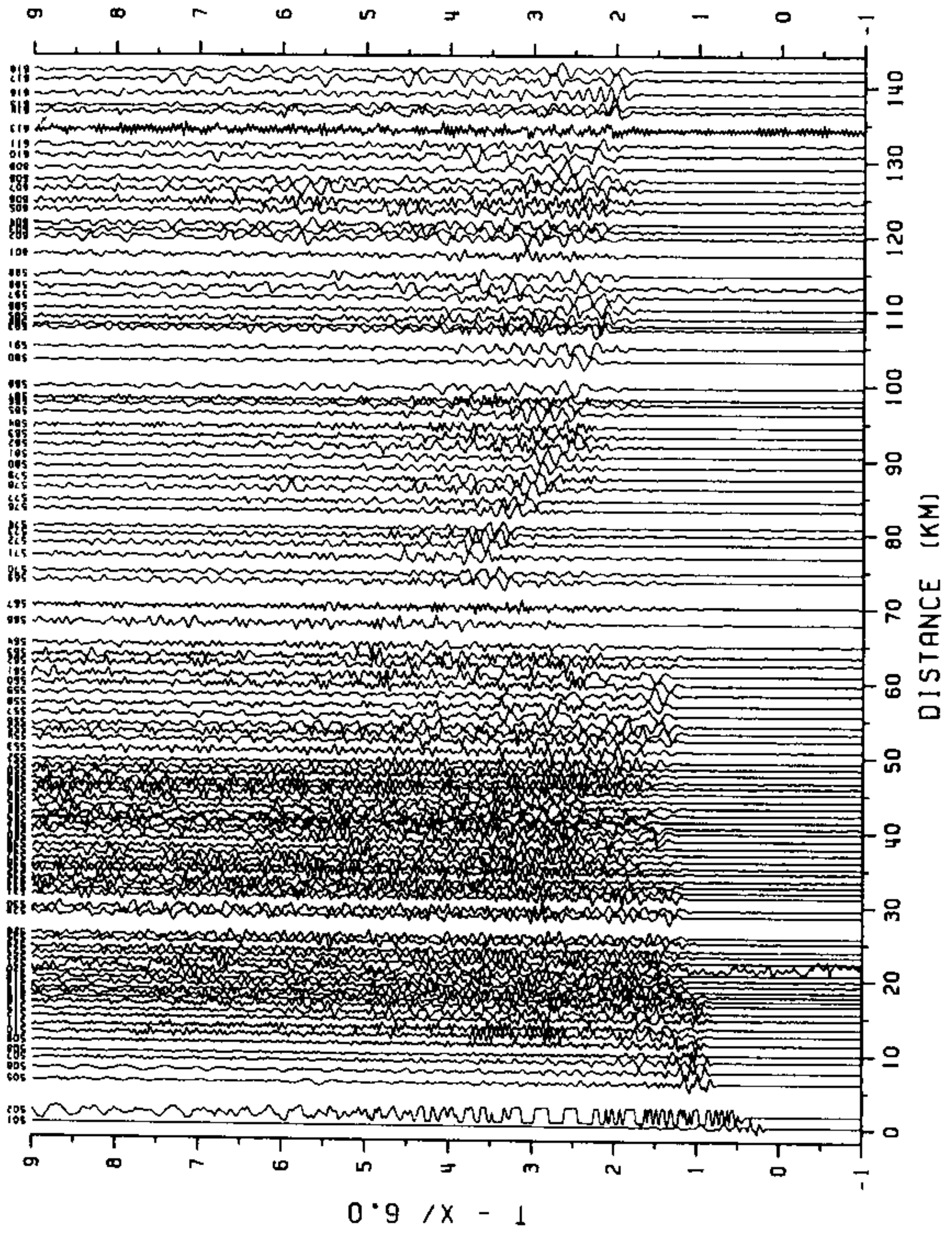
Shot 23, Shotpoint 4
