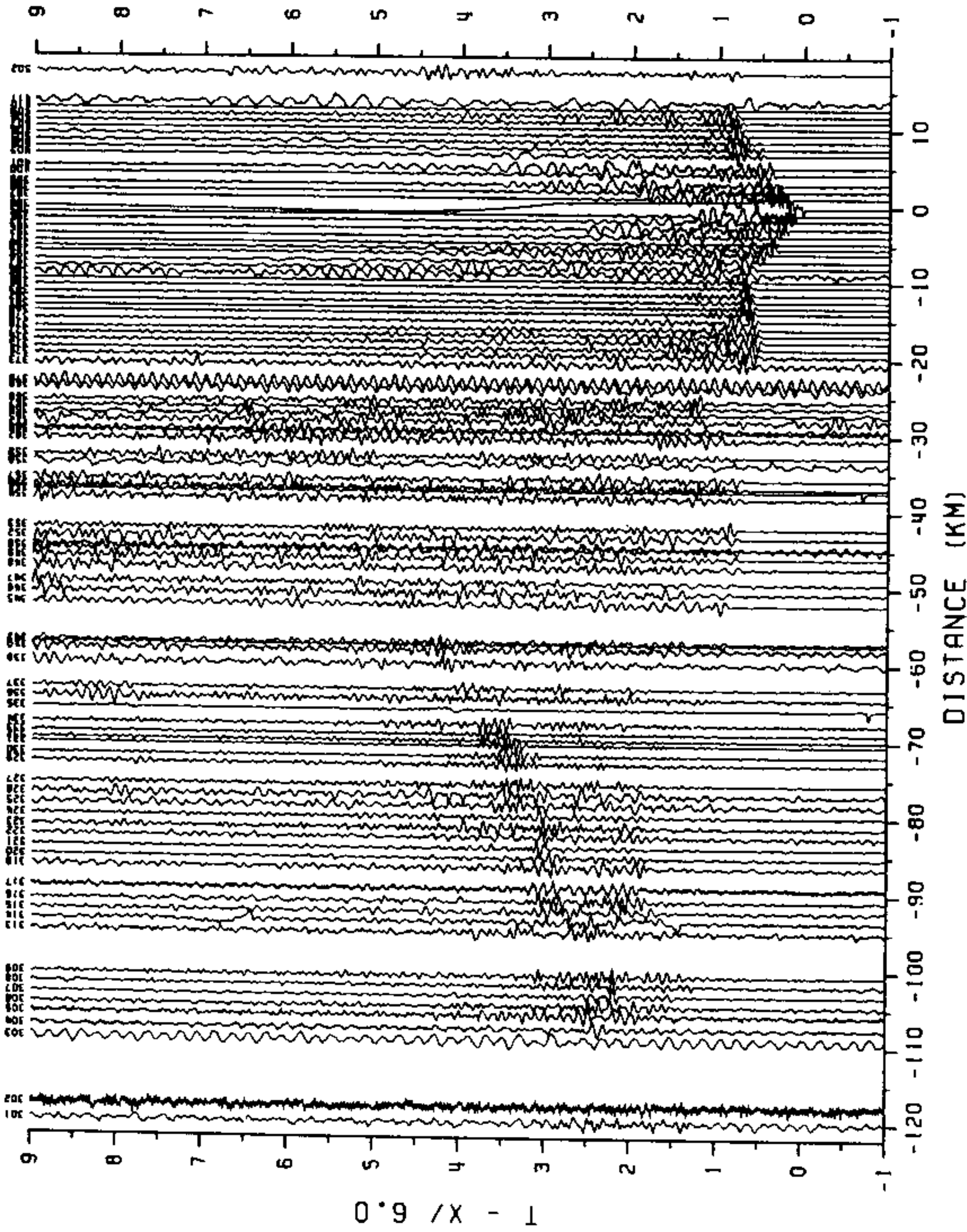
Shot 16, Shotpoint 13
