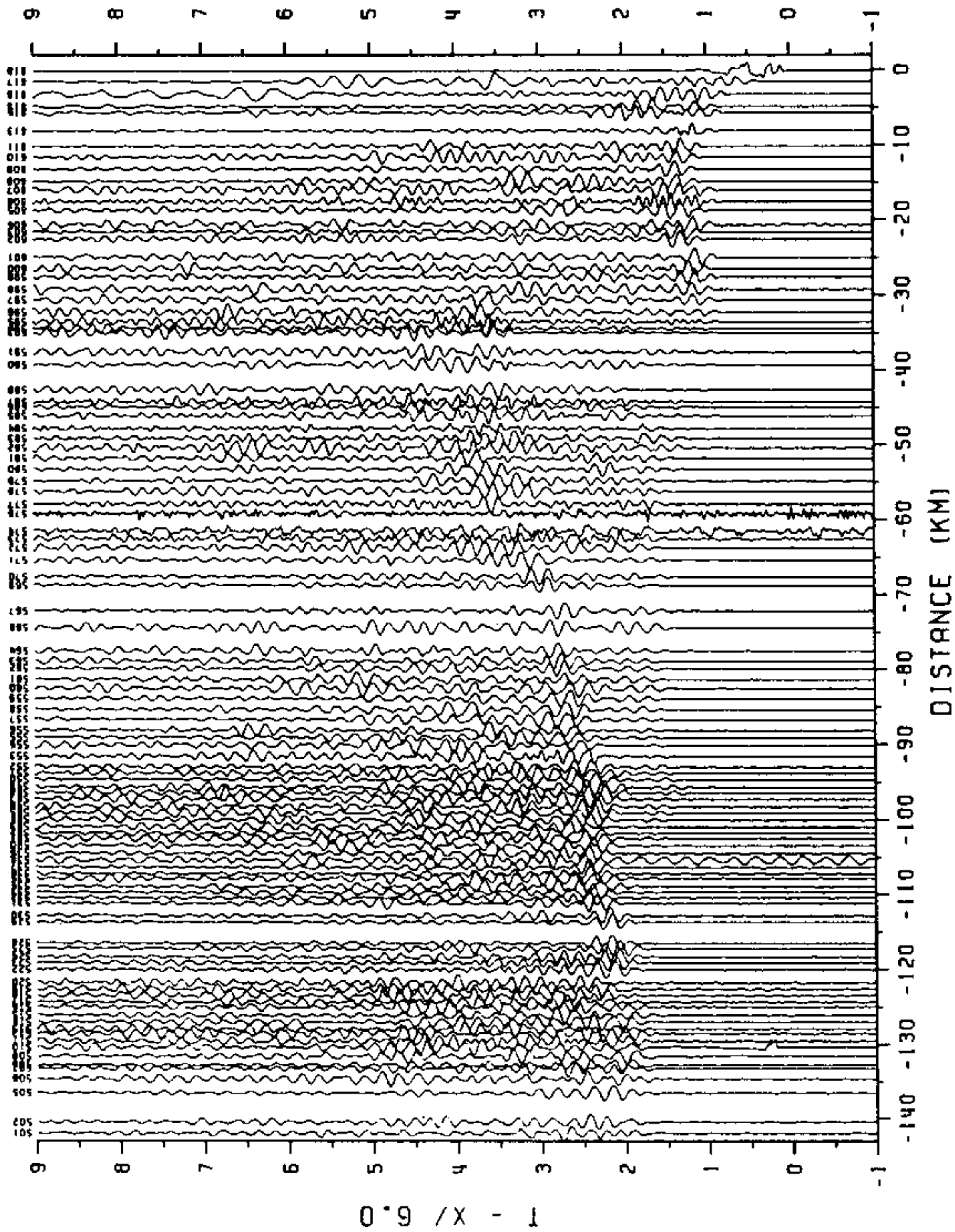
Shot 18, Shotpoint 7
