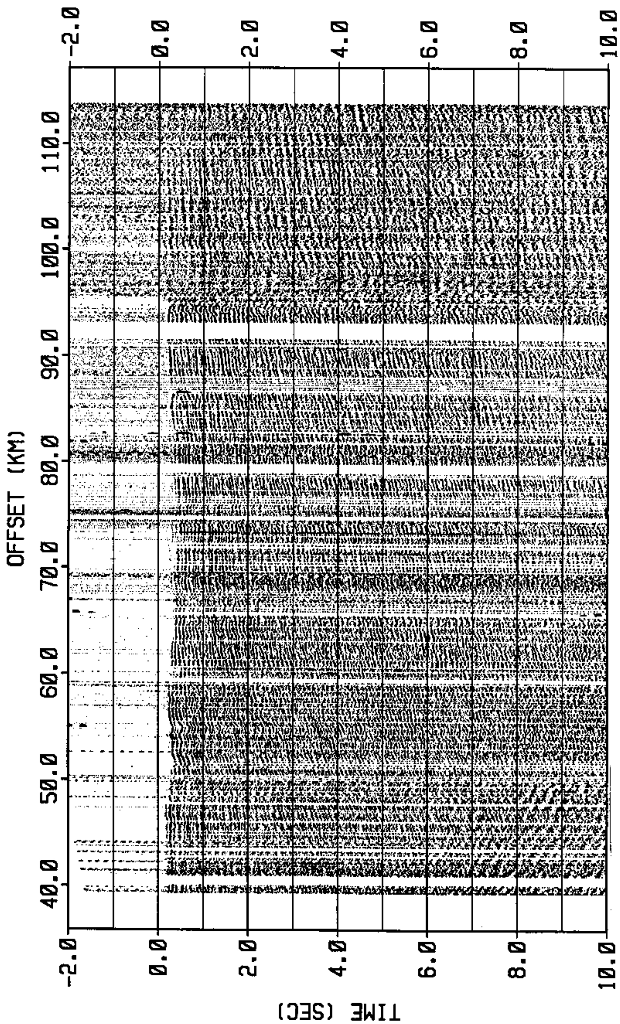
Figure 65 Profile 3 Shot 37 Shot Point 130 AGC = 12 sec
