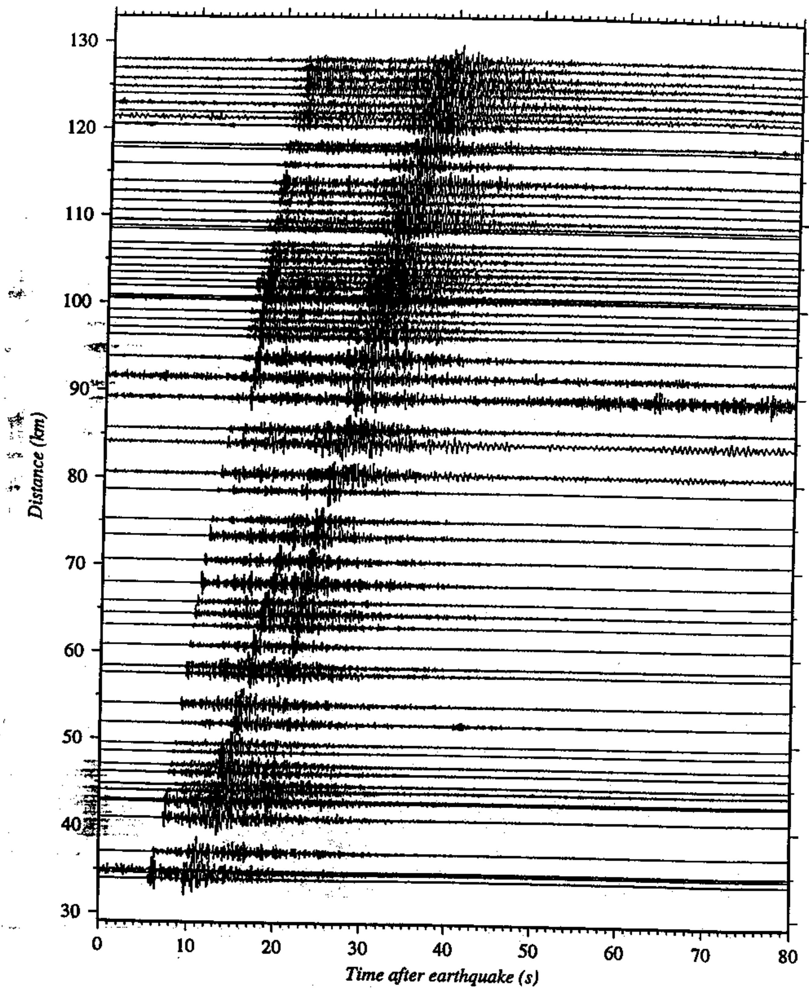
Fig. 7c. Vertical-component record section for local event which occurred on Nov. 24, 1993, 36 km south of Ridgecrest ( M_L=2.7 ). Travel time (unreduced) after earthquake is shown. See text for details.
