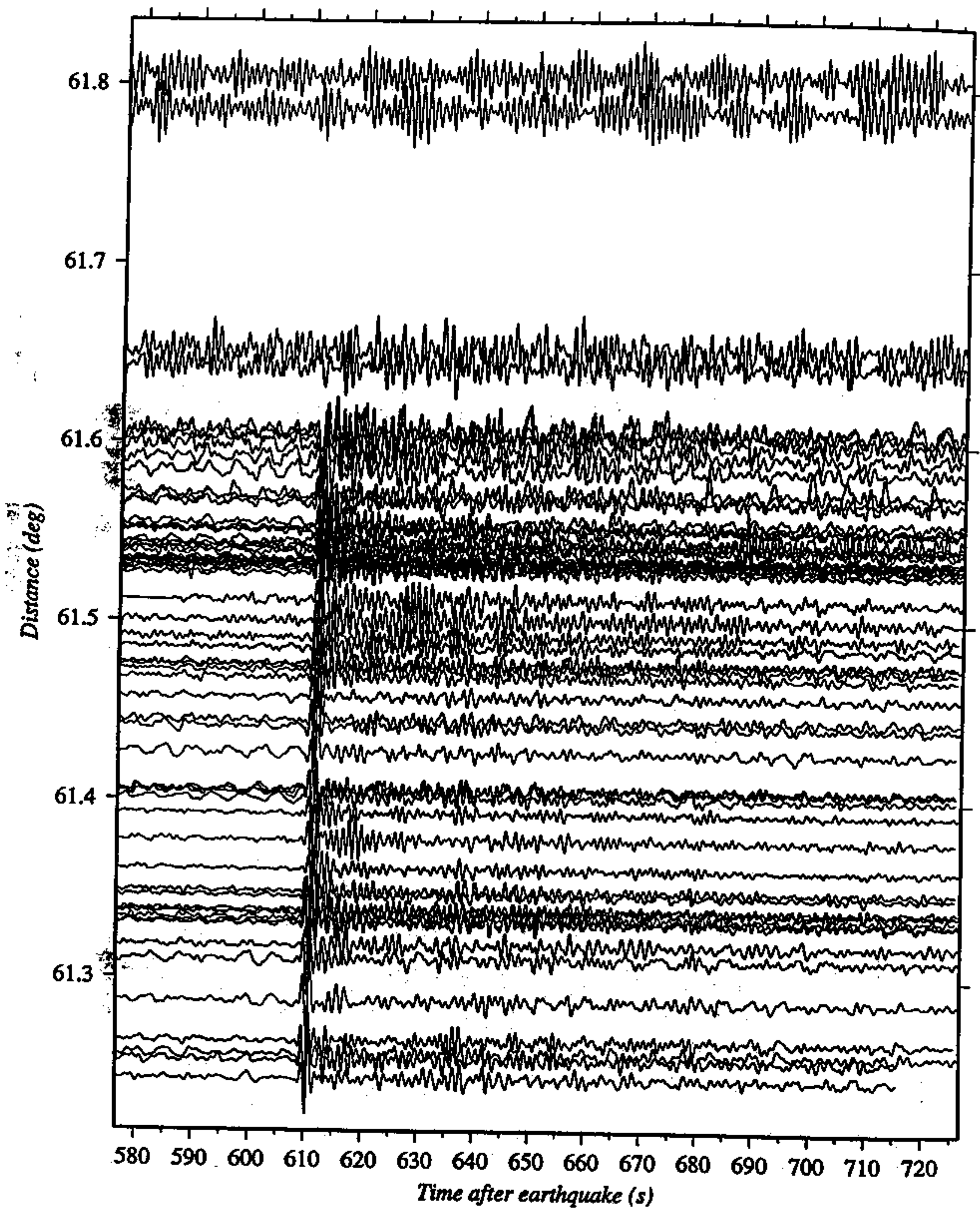
Fig. 6e. Vertical-component record section for teleseismic event which occurred on Nov. 22, 1993 in the Kuril Islands ( m_b=5.1 ). Travel time (unreduced) after earthquake is shown. See text for details.
