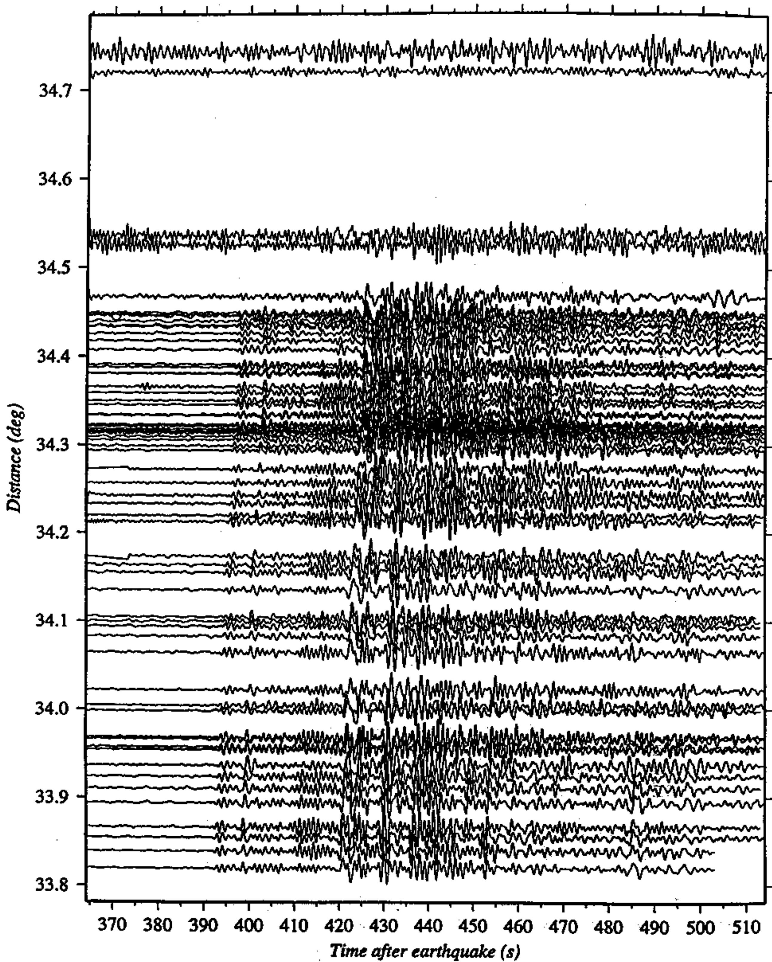
Fig. 6d. Vertical-component record section for teleseismic event which occurred on Nov. 20, 1993 in southern Alaska ( M_w=5.9 ). Travel time (unreduced) after earthquake is shown. See text for details.
