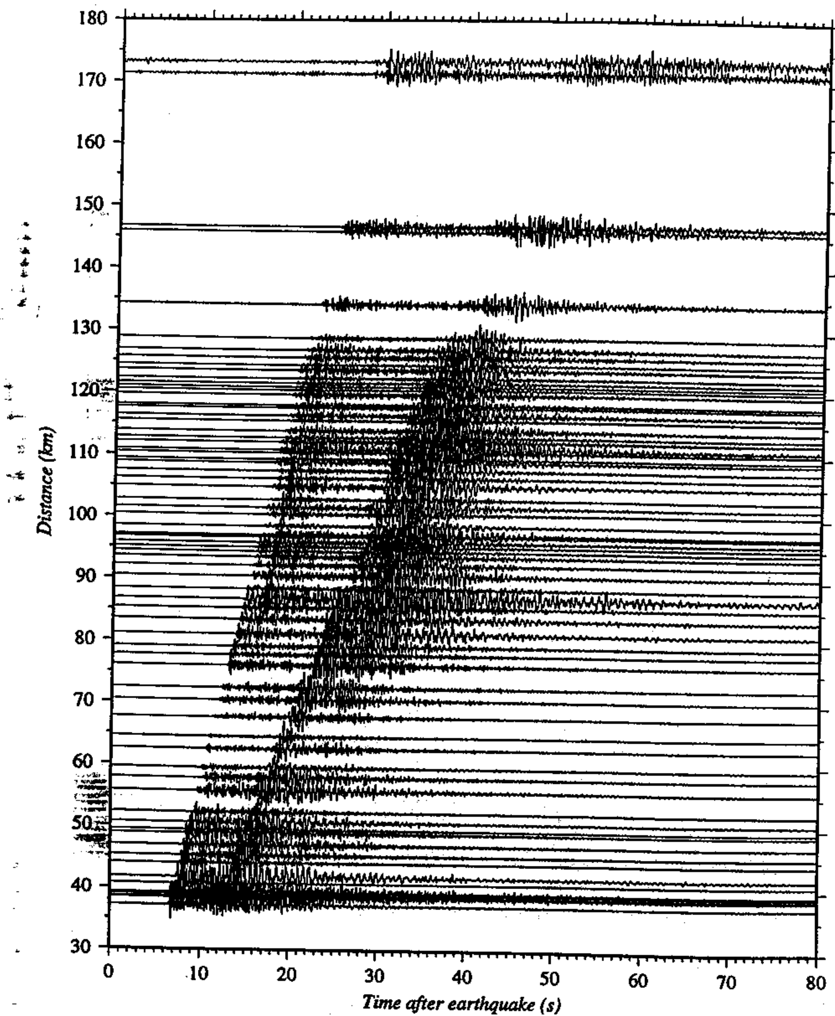
Fig. 7g. Vertical-component record section for local event which occurred on Dec. 8, 1993, 13 km north-northeast of Barstow ( M_L=3.7 ). Travel time (unreduced) after earthquake is shown. See text for details.
