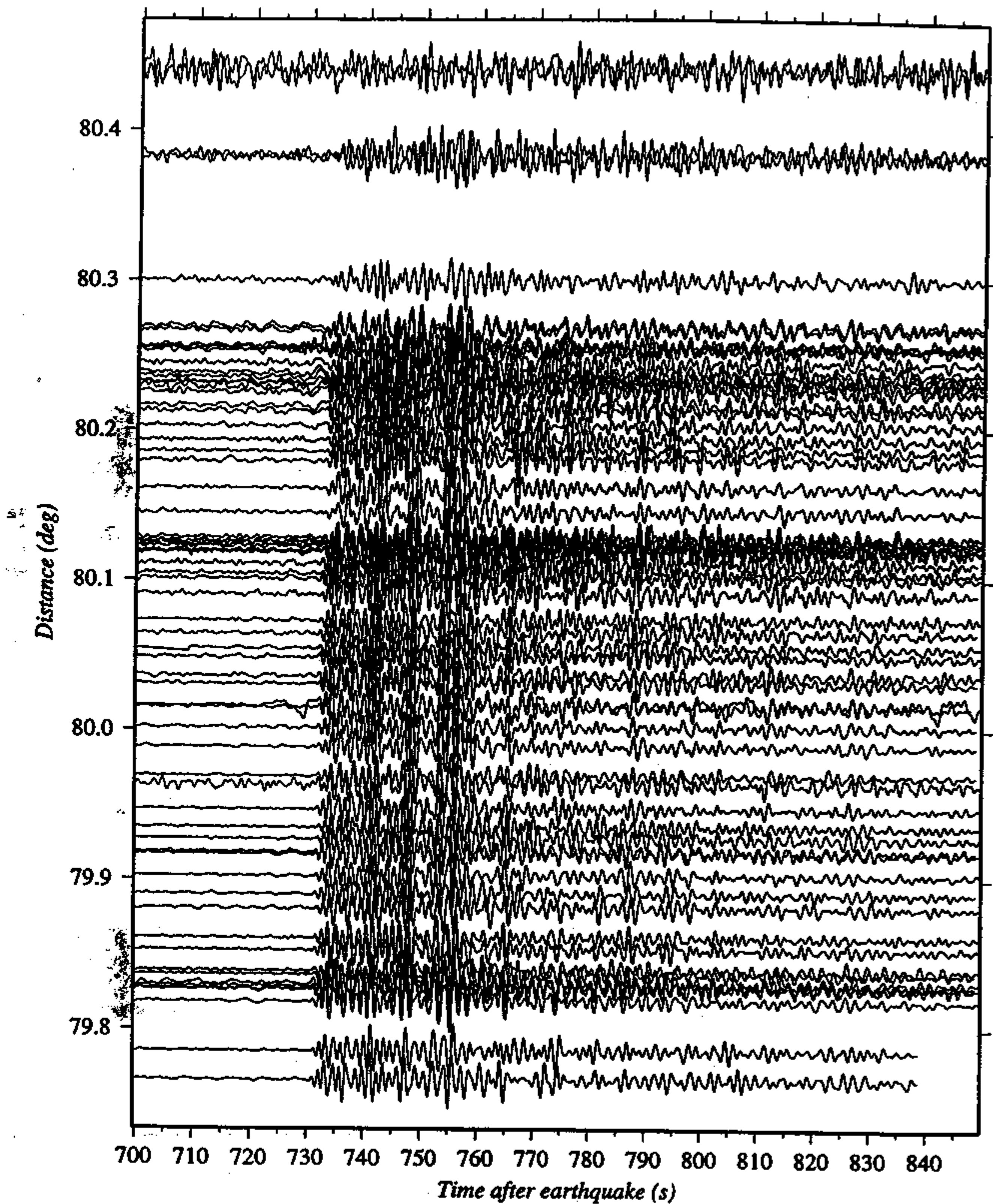
Fig. 6c. Vertical-component record section for teleseismic event which occurred on Nov. 19, 1993 near the central mid-Atlantic Ridge ( M_w=5.8 ). Travel time (unreduced) after earthquake is shown. See text for details.
