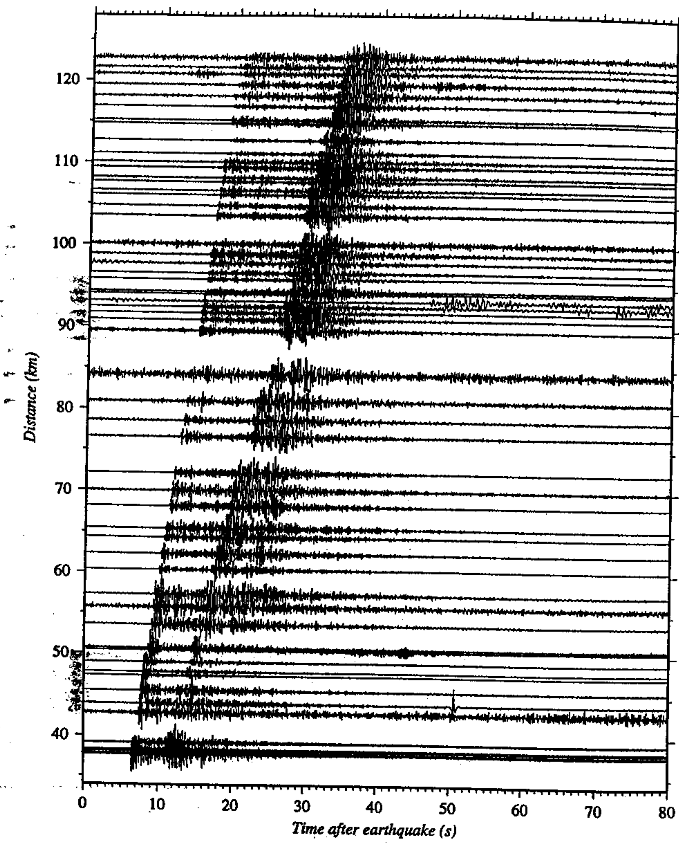
Fig. 7a. Vertical-component record section for local event which occurred on Nov. 22, 1993, 10 km north-northeast of Barstow ( M_L=2.1 ). Travel time (unreduced) after earthquake is shown. See text for details.
