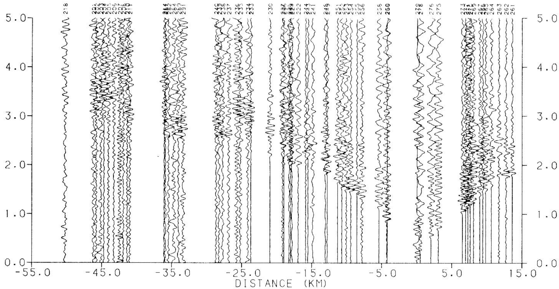
Figure 6. Reduced record section for Livermore shotpoint 1 (shot 2), for the NW-SE profile.
