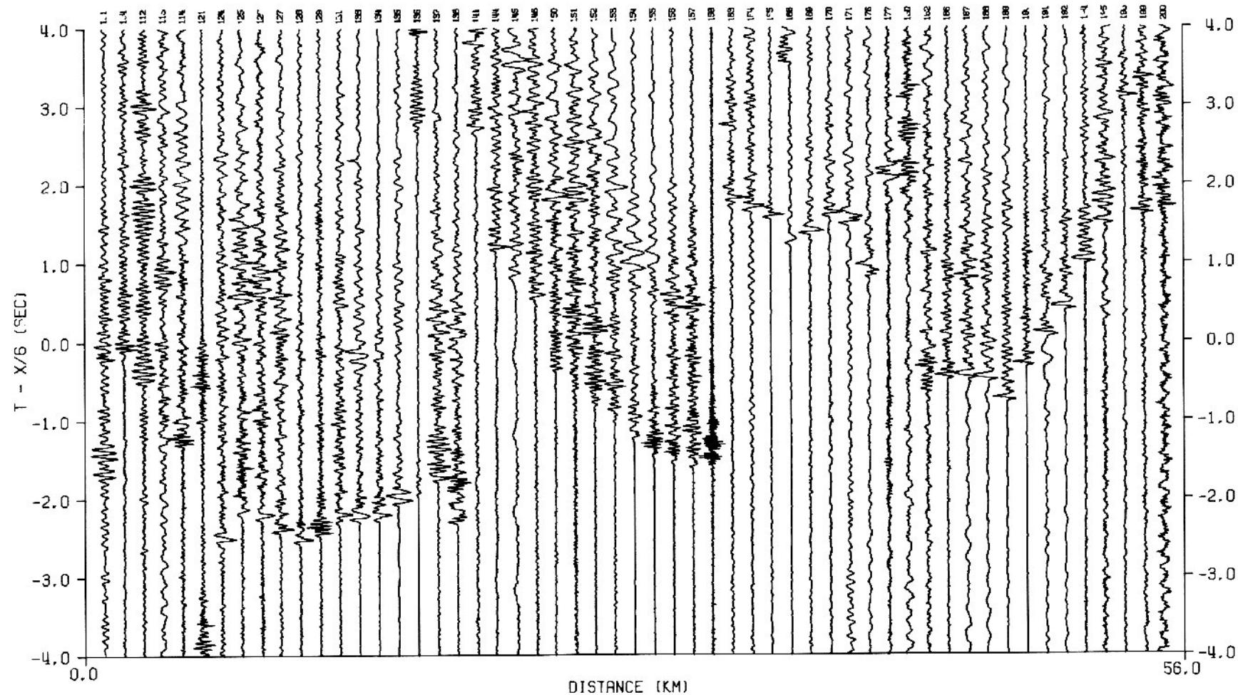
Figure 9. Reduced record section for Livermore microearthquake number 2.
