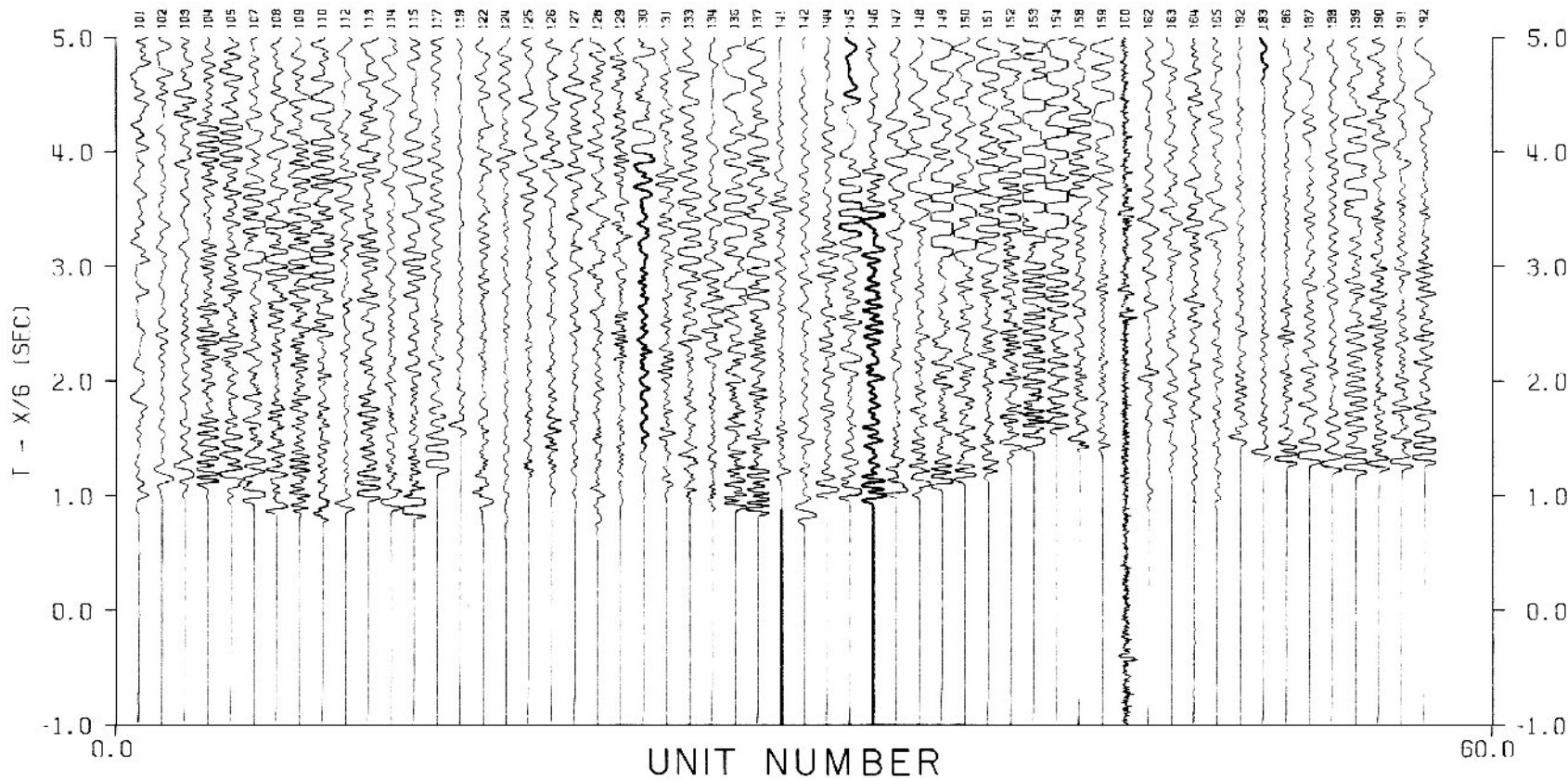
Figure 12. Reduced record section for Livermore microearthquake number 5.
