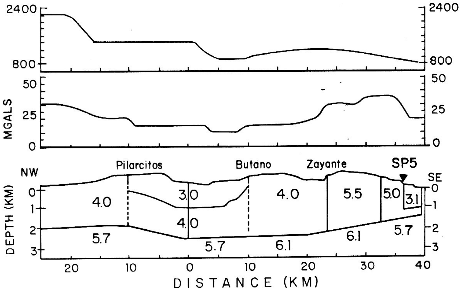
Figure 17. Aeromagnetic profile, gravity profile, and velocity model for the La Honda line from Boken and Mooney (1982).
