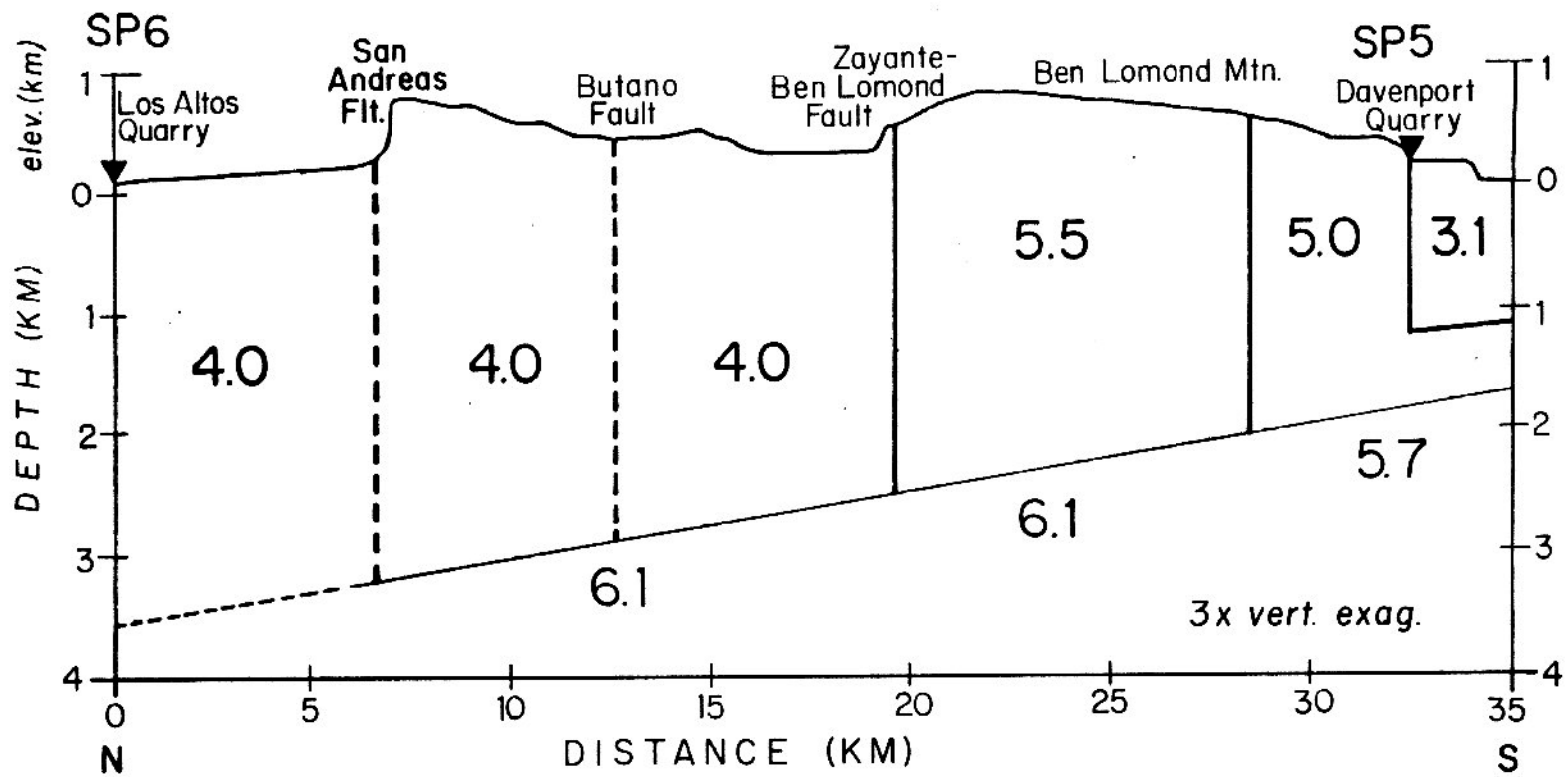
Figure 16. Velocity model prepared by Boken and Mooney (1982). Velocities are shown as kilometers/sec.
