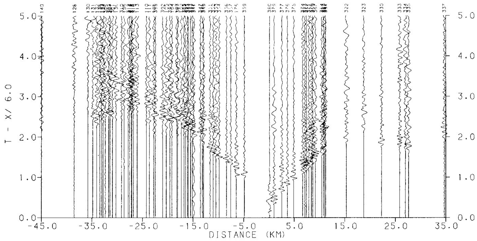
Figure 4. Reduced record section for shotpoint 1 (shot 4), for the north-south profile.
