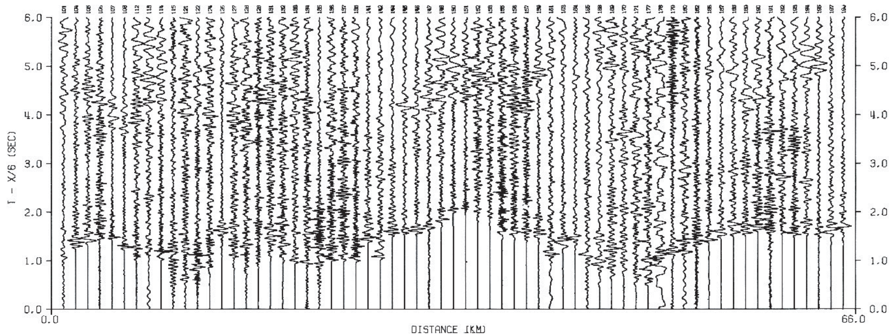
Figure 8. Reduced record section for Livermore microearthquake number 1.
