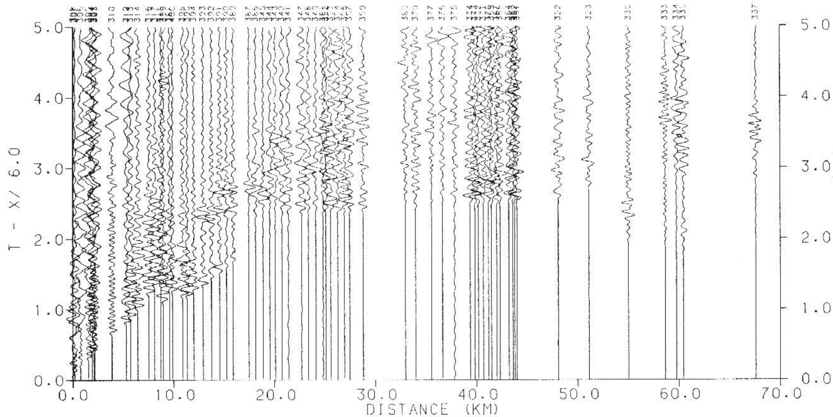
Figure 5. Reduced record section for shotpoint 2 (shot 5), for the north-south profile.
