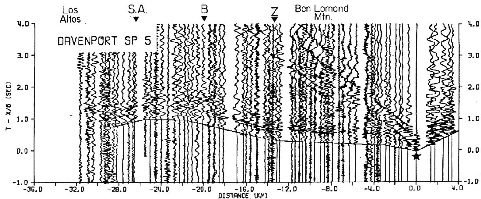
Figure 14. Reduced record sections for Shotpoints 5 and 6 in the Santa Cruz Mountains. Abbreviations: San Andreas fault (S.A.), Butano fault (B), Zayante fault (Z).
