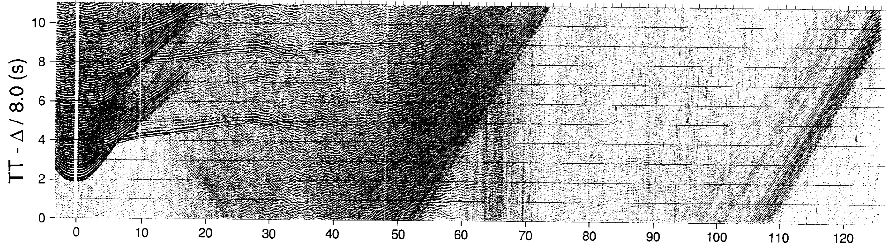
H Vertical component recorded at site 5.
