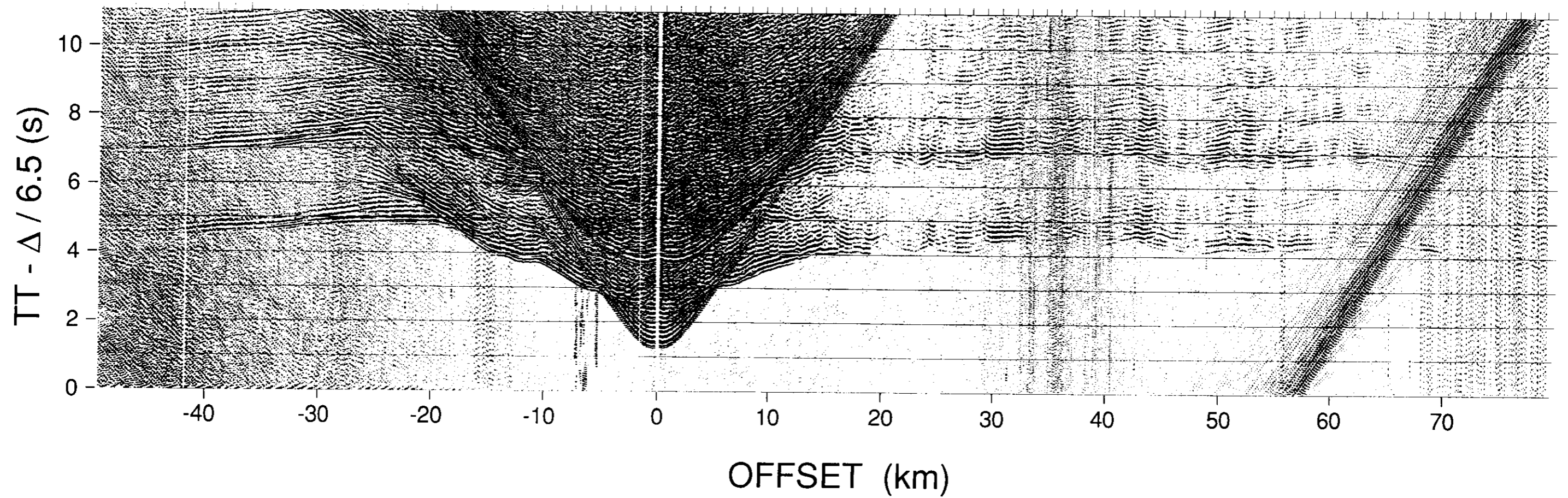
H Vertical component recorded at site 5.
