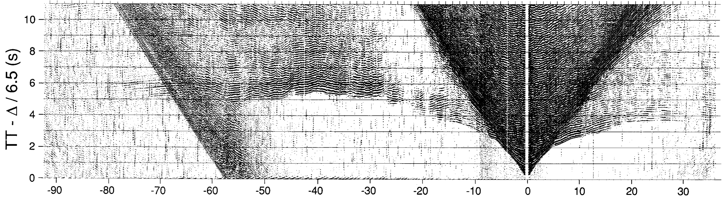
F Vertical component recorded at site 3.
