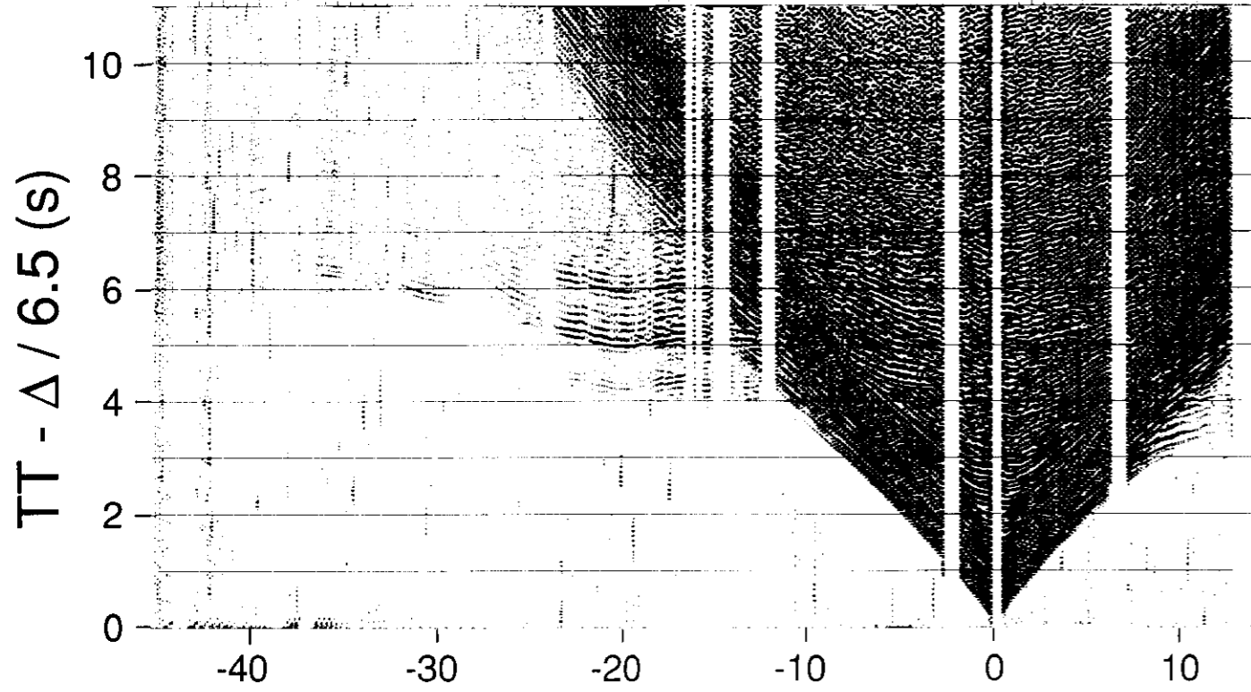
C Radial component recorded at site 2.
