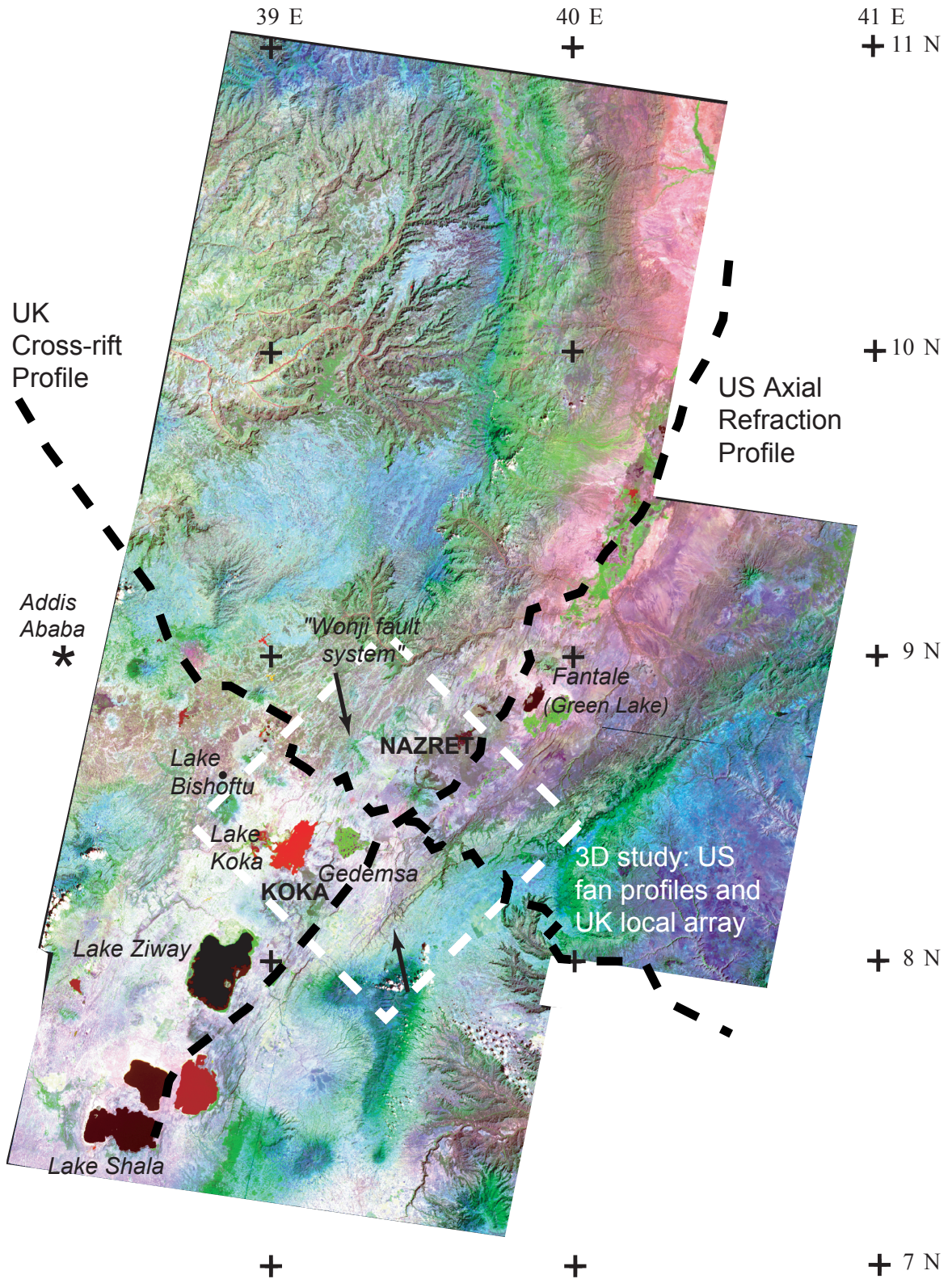
Figure 5. Landsat image of Main Ethiopian Rift.
