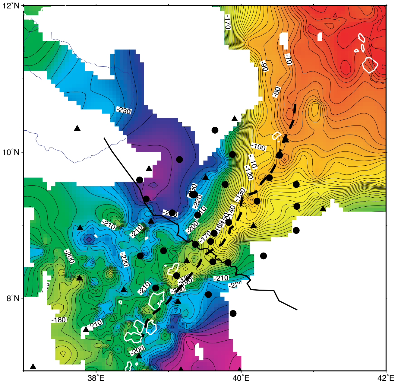
Figure 7: Gravity field over Main Ethiopian Rift. Black line is funded UK refraction profile. Dashed black line is axial refraction profile (funding requested here). Triangles are Andy Nyblade's installed (NSF funded) broadband instruments. Circles are UK (Graham Stuart) installed broadband instruments, which will still be in place in January 2003 to record the wide-angle dynamite shots.
