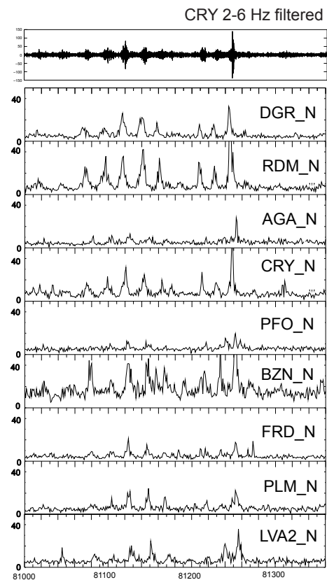
Filtered seismogram (top) and envelope functions of all surface stations that recorded the tremor triggered by the Denali surface waves. Large amplitude bursts are well-correlated in time. Borehole station records are not included in this analysis since most PBO stations were installed after 2006.
