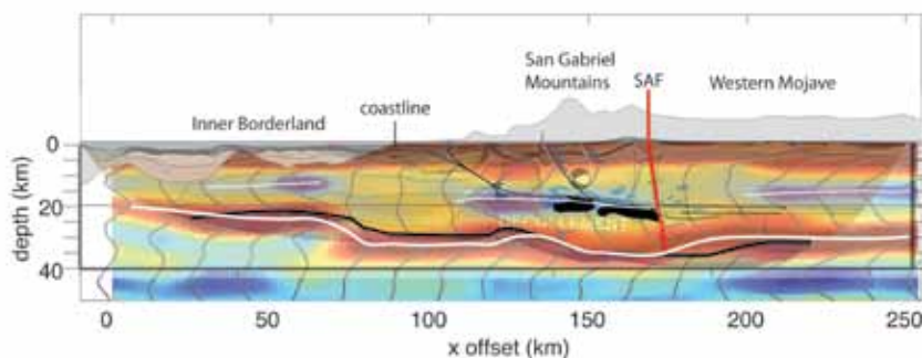
Figure 2. Common Conversion Point (CCP) cross-section for southern California, overlain with results from the LARSE project (Fuis et al. , 2007) to illustrate similarities. In the RF stack, red shading corresponds to positive polarity arrivals and blue to negative. The thick white line represents the RF Moho, while the thick black line represents the LARSE Moho. Thin white lines represent structures (i.e., top of potential shear zones) seen in RFs. The thin black lines represent reflectors interpreted as a decollement in the LARSE cross-section and the thick black bodies represent the LARSE bright reflectors (Fuis et al. , 2007). The thick vertical red line is the projection of the San Andreas fault.
