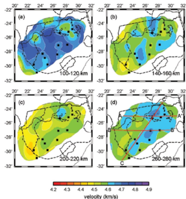
Figure 1. Shear-wave velocity variations at 4 depth ranges. Black squares delineate the sites of kimberlites at 104 to 65 Ma based on Fig. 7c in Jelsma et al. (2004), which show a better correlation with slow regions in shallow upper mantle (a and b). Red lines show the locations of profiles in Figure. 2. Dashed lines are tectonic boundaries.
