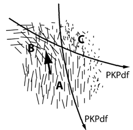
A schematic representation of three distinct anisotropic domains in the IC where the strength and orientation of fast crystallographic axes are shown as straight lines. Two different PKP df ray paths are shown sampling different domains. "A" represents a semi-constant anisotropic domain with a predominant alignment of fast anisotropic axes; "B" is a transitional domain with a mixed orientation of fast anisotropic axes, and "C" is an isotropic or a weakly anisotropic domain. The arrow in the middle represents the net direction of the fast axis of anisotropy.
