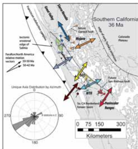
Figure 1. Map of station locations and unique anisotropy axis orientations at 36 Ma based on the reconstruction of McQuarrie and Wernicke (2005). Station color-coding corresponds to the crustal blocks. The large arrows show the best fitting block trend-lines rotated back to their orientation at 36 Ma. The rose diagram shows the number of stations with anisotropy trends within each 10° bin when rotated back to their 36 Ma orientations. Vectors show Early Tertiary Farallon-North America relative motion vectors.
