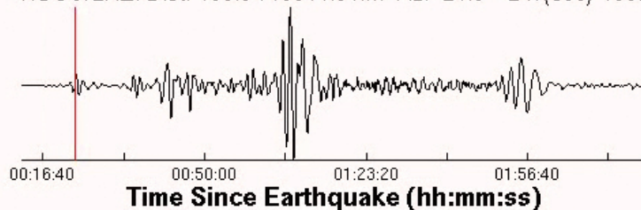
Ground Motion Visualization (GMV) of the April 6, 2009 earthquake of Northern Sumatra, Indonesia.
