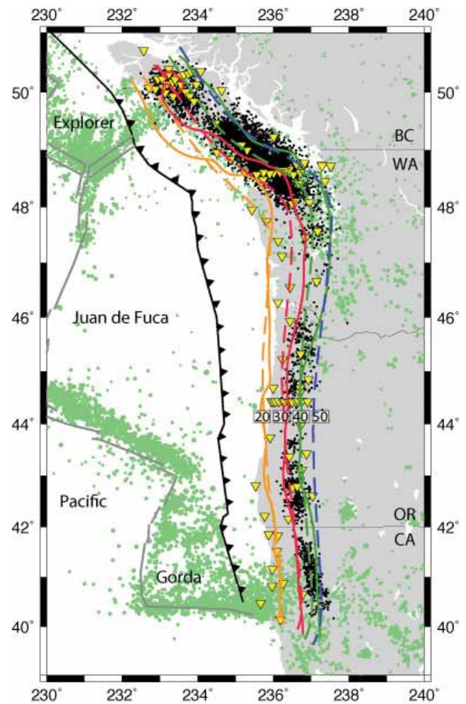
Depths contours of the top of the plate interface from receiver functions (this study, solid lines) and a compilation of various studies (dashed lines, McCrory et al., 2006) along the Cascadia margin. Earthquake epicenters from the GSC and USGS catalogues for M > 2 are shown as black dots; tremor epicenters appear as inverted yellow triangles. Numbers indicate depth (in km) to each contour. Solid black line with arrowheads indicates the location of the trench offshore.
