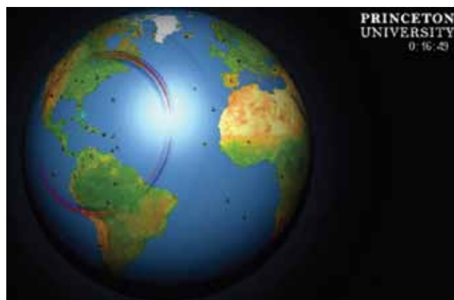
Snapshot of a spectral-element simulation of the January 12, 2010, Mw = 7.1 Haiti earthquake. The near real-time system produces animations of all earthquakes reported by the Global CMT Project. The animations show the velocity wavefield on Earth's surface as a function of time. Red: upward motion; Blue: downward motion. The prominent waves are the Rayleigh surface waves, and one can vaguely see SS waves crossing, e.g., Greenland.
