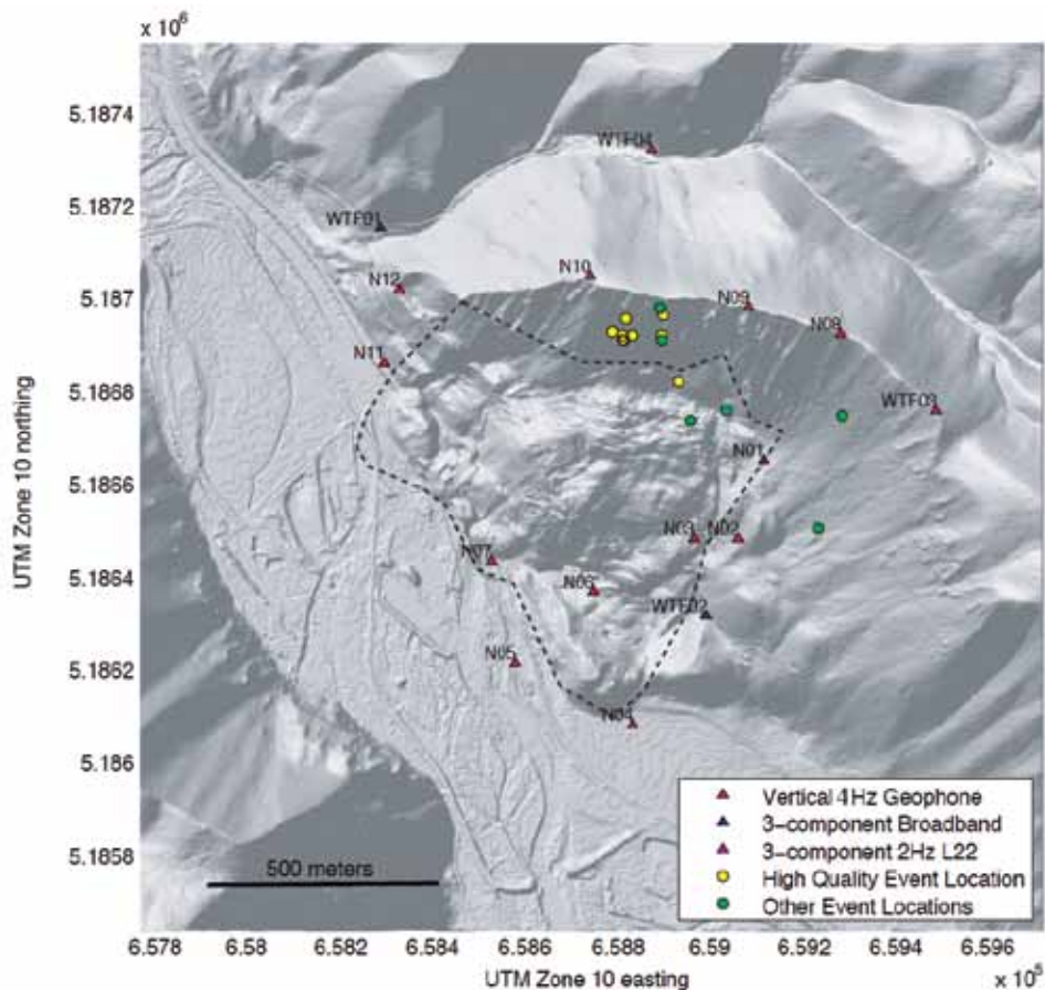
Lidar image of the Nile Valley Landslide with location of stations installed after the slide (triangles) and best-fit post-slide event locations (circles). The dashed line indicates the approximate boundaries of the landslide and uplifted areas at the toe. Lidar image provided by Washington State Department of Transportation.
