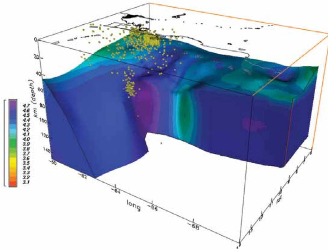
Surface wave tomography model illustrating the structure of the South American mantle lithosphere as viewed from the northwest. The yellow dots are relocated seismicity, which define the Paria cluster and the location of the subducted oceanic lithosphere beneath the Antilles arc tearing away from the continental lithosphere along the Caribbean-South American plate boundary.
