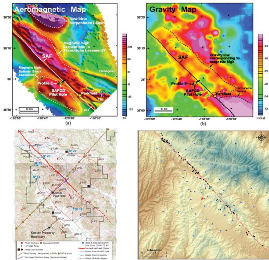
Figure 3.2. Detailed geophysical surveys in the vicinity of the SAFOD site.
