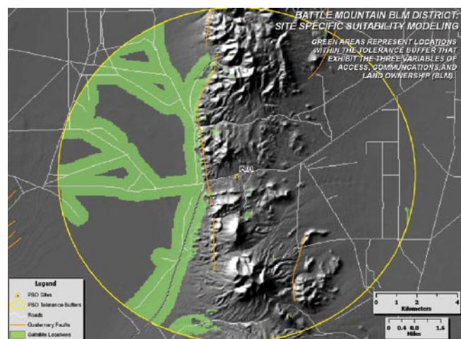
Figure 1.3. Triangle indicates the GPS station location chosen by siting committee. Yellow circle shows stations siting buffer. Green shading indicates suitable station location based on station access, land ownership, and cellular modem coverage. Station was built due south of triangle.
