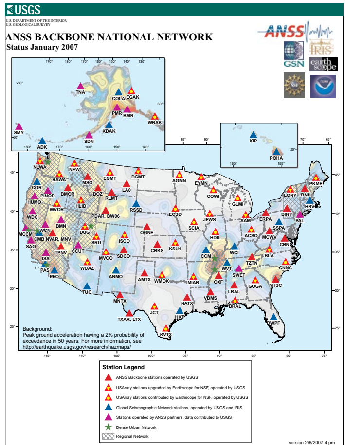
Figure 2.1. The ANSS Backbone as of January 2007. Stations with yellow centers were contributed by USArray. EarthScope will continue to work with the USGS to fill the remaining gaps in the central United States to complete the Reference Network.
