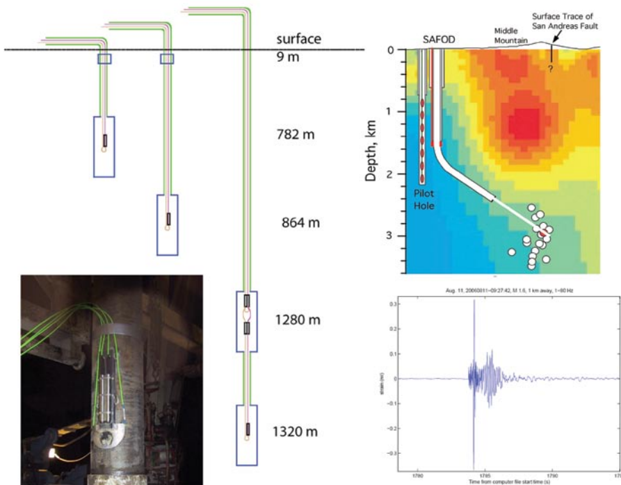
Figure 3.6. Illustrations of the deployment of the fiber optics laser interferometer installed behind cemented casing by Mark Zumberge of University of California San Diego and an example of strain data resulting from a nearby microearthquake.
