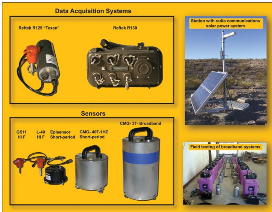
Figure 2.4. Shown here are the major components that constitute the equipment for the Flexible Array. The single-channel Reftek R125 "Texan" data acquisition system is paired with a 4.5 Hz GS11 or 40 Hz L40 vertical sensor. The three-channel Reftek R130 data acquisition system can be used with either the CMG 40T-1Hz short-period sensor or the CMG 3T broadband sensor. Many Flexible Array stations are equipped with radio communications equipment that can be arranged into a real-time seismic network. Solar power systems, enclosures, sensor vaults, and shipping cases comprise the ancillary equipment for a Flexible Array station.
