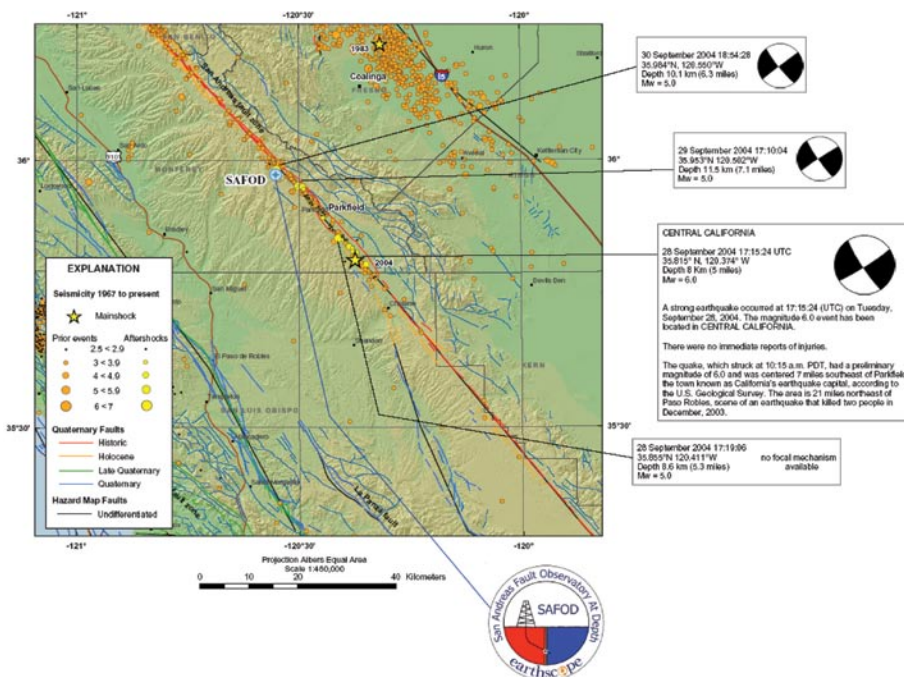
Figure 3.1. The location of the SAFOD site and seismicity along the San Andreas Fault and in the surrounding region. Epicenters of the 2004 Parkfield main shock and the two largest aftershocks are shown.
