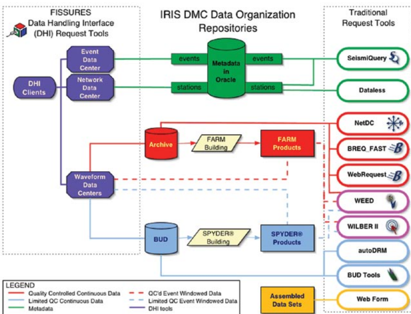
Figure 2.6. Request mechanisms and data repositories at the IRIS Data Management Center. Seismic waveforms and metadata are stored in the real-time and archival repositories shown in the center part of the figure. All EarthScope seismic data are available through the standard DMC request tools (right side) and the Data Handling Interface (DHI) (left side).
