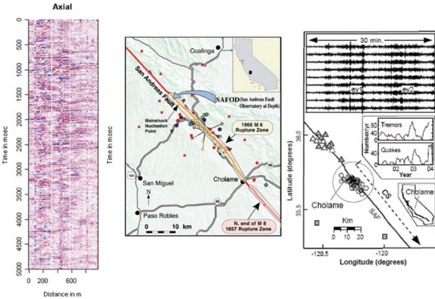
Figure 3.5. Non-volcanic tremor recorded on the PGSI array are shown on the left. This event is associated with slip at depth in the Cholame area. The figure on the right is from Bob R. Nadeau and his colleagues.
