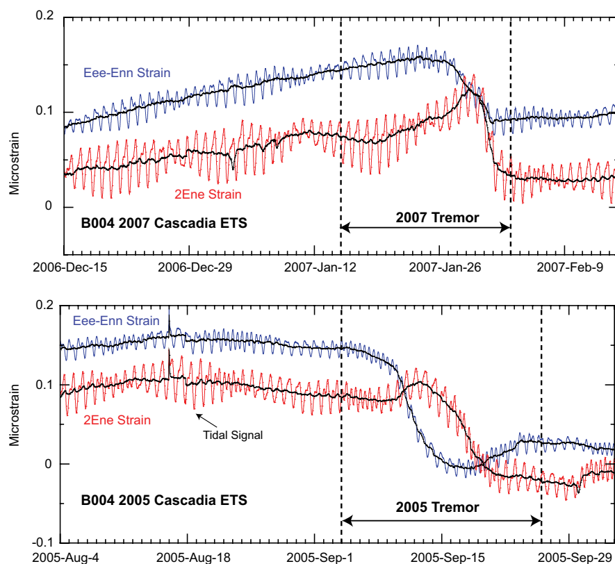
Figure 1.11. Example of strain data products produced by the BSM Analysis Center. Both subfigures show time series of shear strain from PBO borehole strainmeter station B004, which was installed on the Olympic Peninsula in June 2005. This station, the first installed in the PBO network, recorded strain transients associated with the 2005 (bottom) and 2007 (top) episodic tremor and slip events in the Cascadia subduction zone. Red and blue lines in both figures show shear strain with solid Earth tides, while black lines show the same series with solid Earth tides removed. The data have been detrended and the atmospheric pressure effect removed. Values in both cases are in microstrain (one part per million), and both figures span approximately two months of data.
