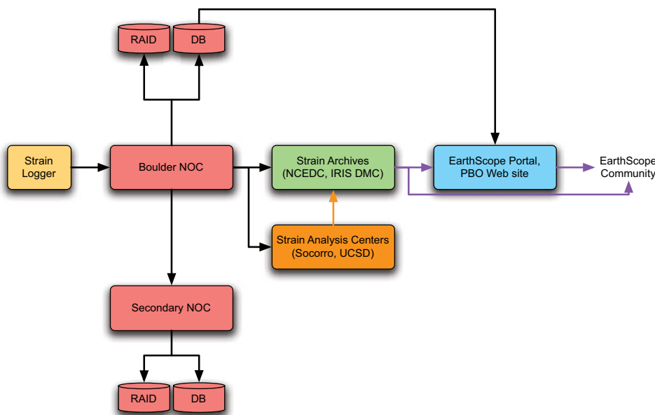
Figure 7.3. Flow of data through PBO Strain Data Management System. The Boulder Network Operations Center (NOC) downloads data from strainmeter stations, copies the data to a local RAID system, extracts necessary meta-data into the PBO Operational Database (DB), and transmits data to the PBO strain archives at the Northern California Earthquake Data Center (NCEDC) and IRIS Data Management Center (DMC). The Boulder NOC will also mirror these data to the secondary NOC on a routine basis; the secondary NOC can take over all critical operations of the Boulder NOC in the event of system failure in Boulder. The Boulder NOC also delivers data to the PBO strain analysis centers at Socorro, NM (borehole) and University of California, San Diego (laser strain), which create Level 2 products that they send to the strain archives. Users can access PBO strain data products from the archives through a number of mechanisms, as well as via the PBO Web site and the EarthScope Portal. See sections 2.3.3.5 and 2.3.3.6 for more details.
