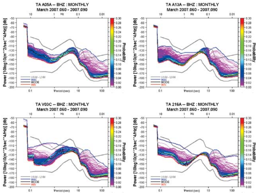
Figure 4.13. Examples of the noise performance (power spectral density plots) for typical Transportable Array stations. The range of noise levels over a one month time interval is shown. The brighter colors indicate the most probable levels; outliers indicate less frequent changes in signal level due to wind, traffic, or earthquakes. The microseismic peak near 8 sec is typical of continental stations. The noise levels over the entire range shown compares favorably with the performance of other permanent stations of the GSN and ANSS.
