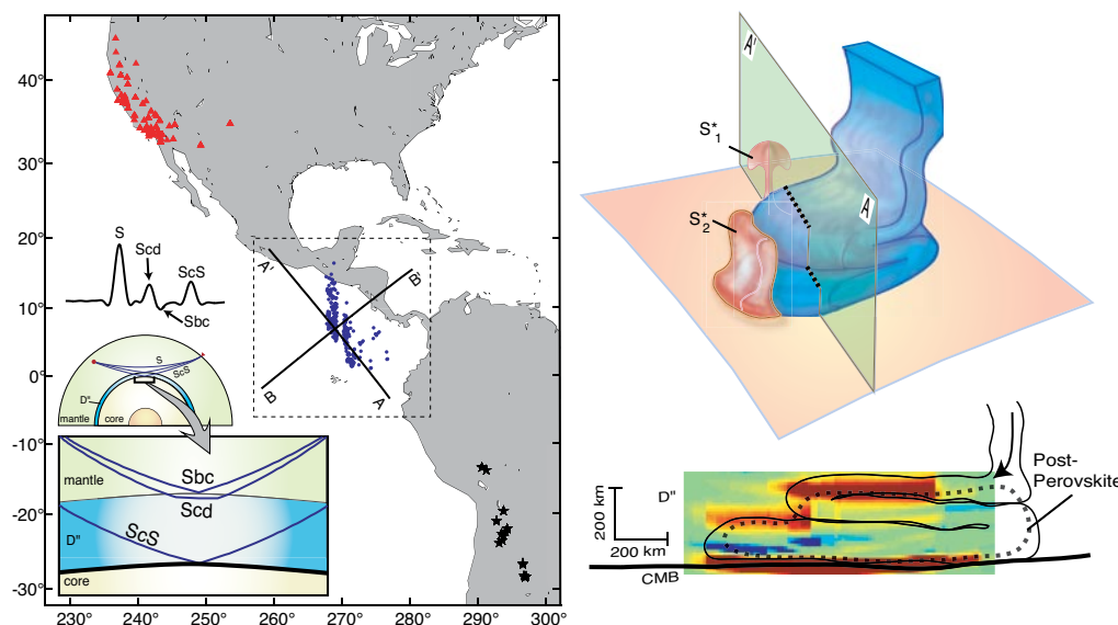
Figure 3.6. An example of use of USArray Transportable Array and broadband regional network data to study lower-mantle structure below North America. The deep mantle corridor sampled by paths from deep South American events to the initial Transportable Array deployment in the western United States is shown on the left. S and ScS observations were migrated to form the image on the right along profile A-A', which is interpreted as having a reflector above the core-mantle boundary caused by post-perovskite phase transition in a cold, folded and piled relic Farallon slab. From: Hutko, A. R., T. Lay, E. J. Garnero, and J. Revenaugh. 2006. Seismic detection of folded, subducted lithosphere at the core-mantle boundary. Nature 441:333-336.
