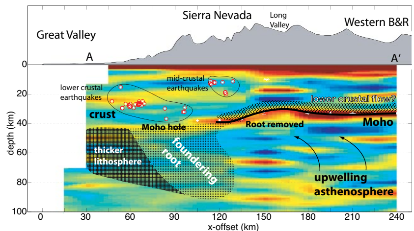
Figure 3.2. Example of deep crust and uppermost mantle imaging achieved by passive-source seismology using portable deployments of USArray Flexible Array instruments (SNEP project). This is a southwest-northeast oriented cross section across the Sierra Nevada with receiver functions and interpretations. Surface topography along this profile is plotted along the top of the cross section. Red colors correspond to positive polarity arrivals while blues mark negative polarities. Earthquakes located near this profile are plotted as white asterisks within red circles. An interpretation of flow within the lower crust is based on observations of anisotropy at the base of the crust towards the eastern part of the array (Frassetto et al., 2006). The lack of a Moho arrival along the southwestern portion of the cross section can be explained by a gradual increase in seismic velocities between the base of the crust and the still-intact portion of the batholithic root. The bright Moho present to the northeast marks the sharp contrast between the crust and inflowing asthenosphere that replaces the root following removal. Courtesy of H. Gilbert, C. Jones, and G. Zandt.
