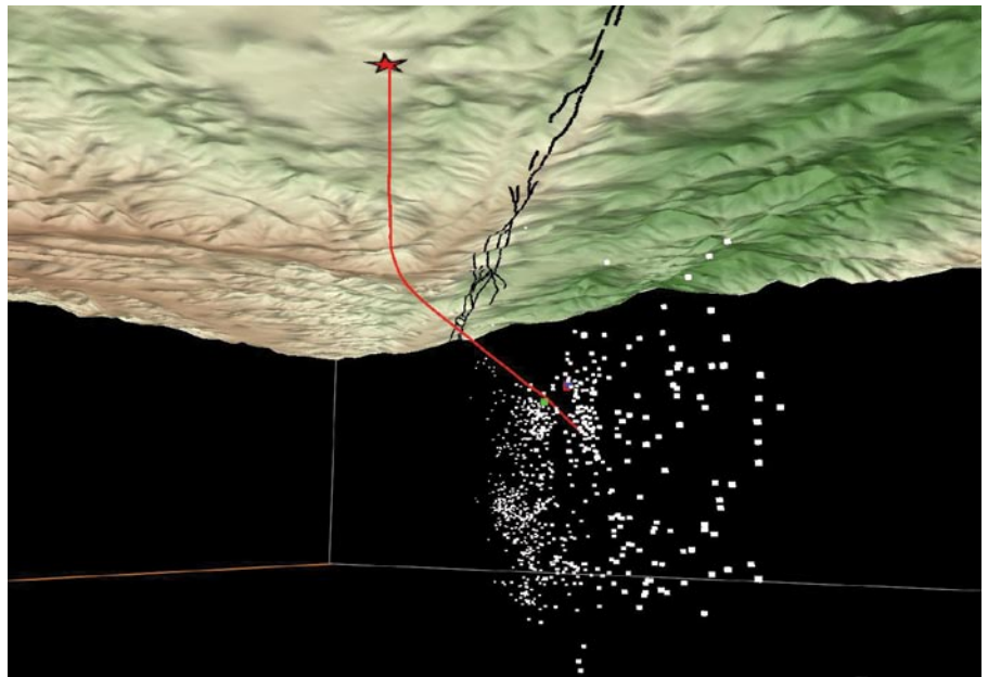
Figure 3.12. Seismicity of the San Andreas Fault as seen from a vantage point in the earth looking to the northwest. Hypocenters were determined by the Parkfield Area Seismic Observatory (PASO) UNO, PASO DOS, and EarthScope Flexible Array (PASO TRES) experiments, courtesy of Steve Roecker (RPI) and Cliff Thurber (University of Wisconsin). The San Andreas Fault is made visible by more than 1000 microearthquakes observed by the PASO networks. The SAFOD main hole is shown in red, extending downward from the surface facility (star). The surface trace of the fault is shown in black draped over the topography. The absolute locations of the SAFOD target earthquakes (red, blue and green symbols) were determined using travel time observations from instruments in the SAFOD main hole; PASO TRES, U.C. Berkeley HRSN and USGS NCSN network data; and active-source seismic experiments (recorded downhole and on the surface networks) conducted in 2004, 2005, and 2006.
