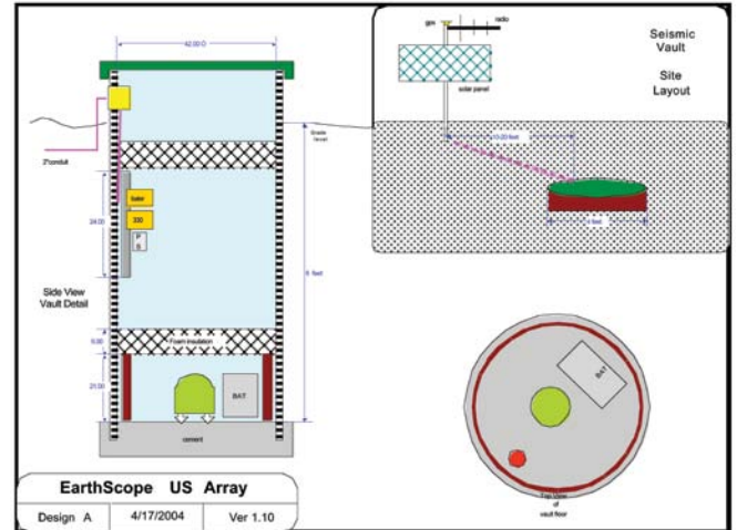
Figure 4.14. Details of the standard site vault developed for Transportable Array stations. Photographs of installation and sites are shown in Figure 2.2.
